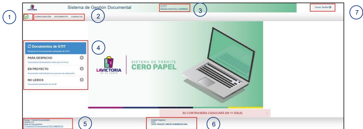
Figura 3. Pantalla Principal
